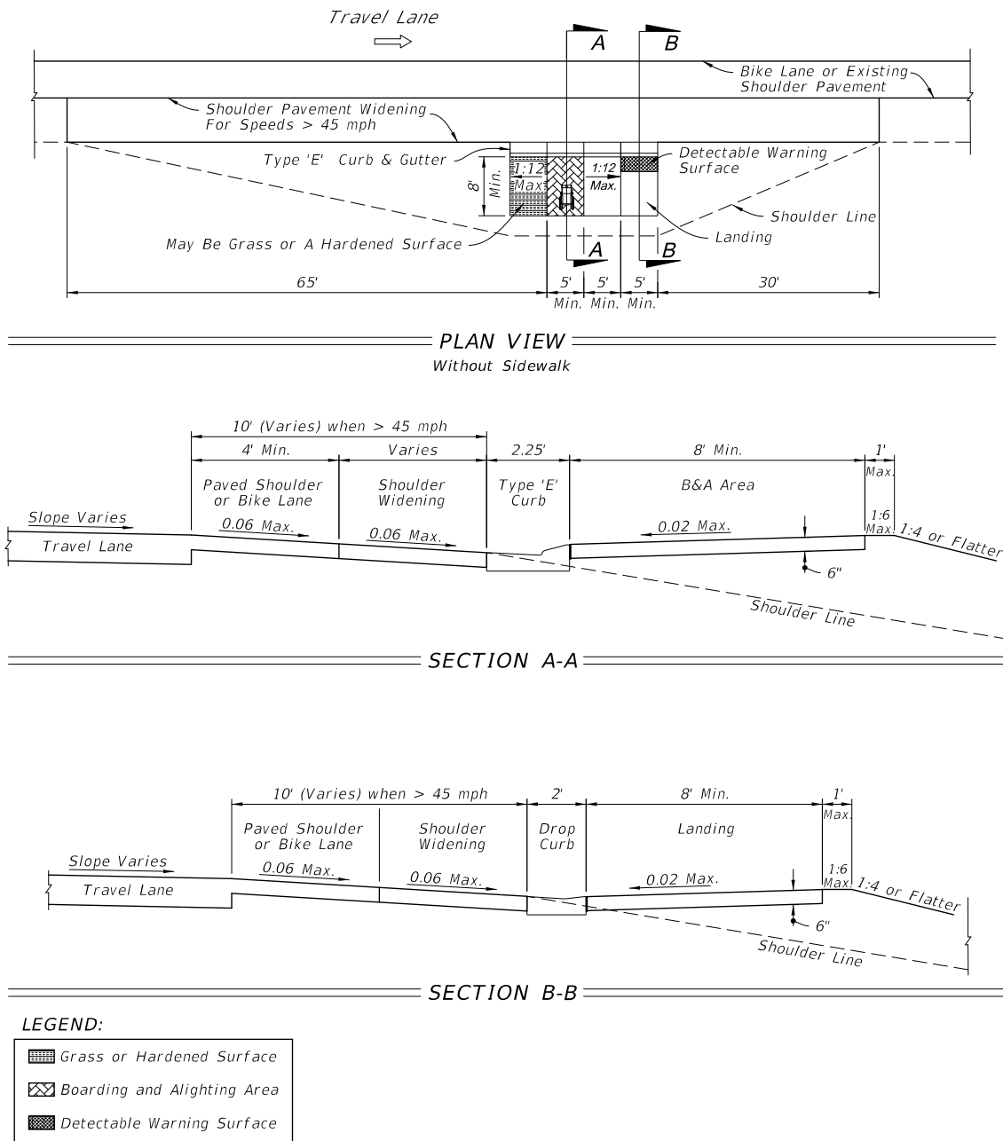
Figure 13 – 1 Boarding and Alighting Area for Flush Shoulder Roadways with Connection to the Roadway
